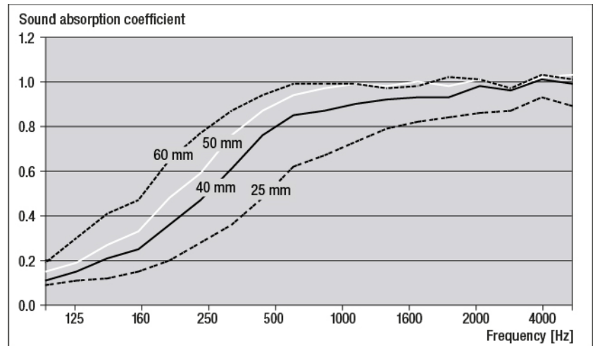
Diagram 3: Degree of sound absorption of Basotect® B as a function of the thickness, according to DIN EN ISO 354 (reverberation room)
