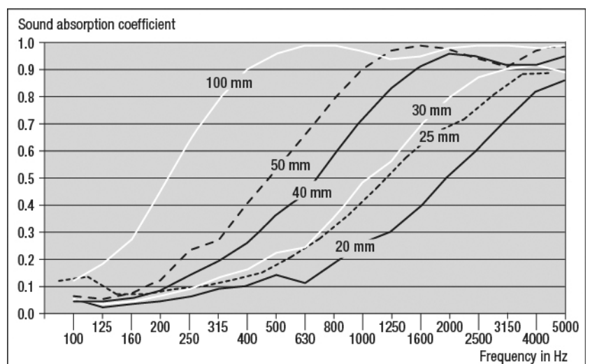
Diagram 2: Degree of sound absorption of Basotect® B as a function of the thickness, according to ISO 10534-2 (impedance tube).
